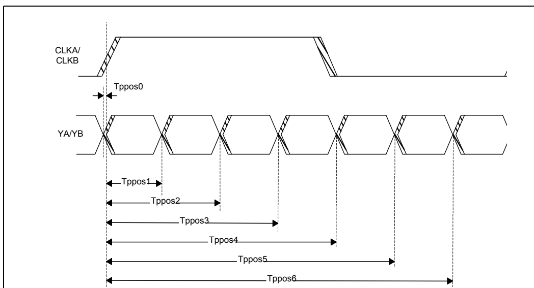
Figure 8-11. Clock Timing
